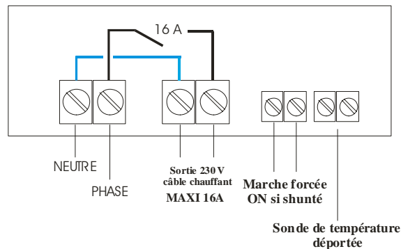
THERMOSTAT NOVATRACE THA/E
